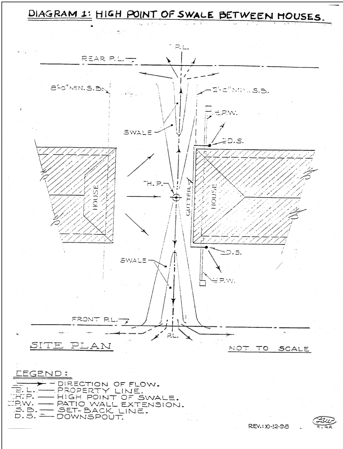
Diagram 1: High Point of Swale between Houses
