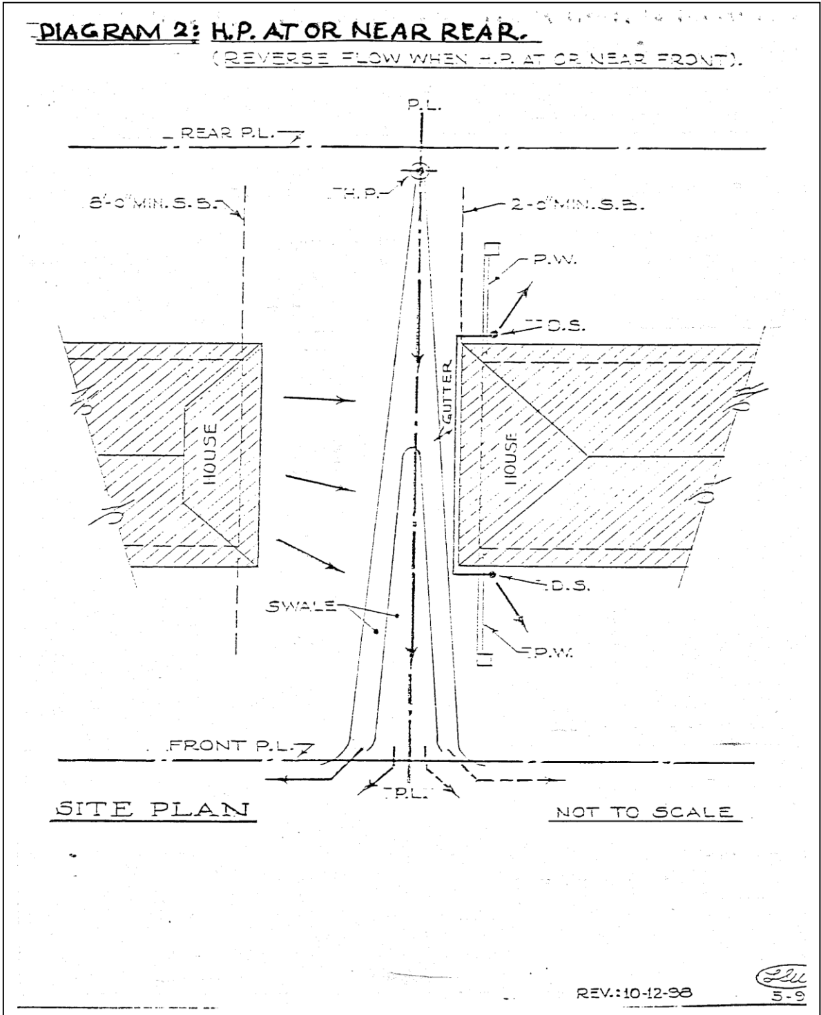
Diagram 2: High Point at Near Rear
