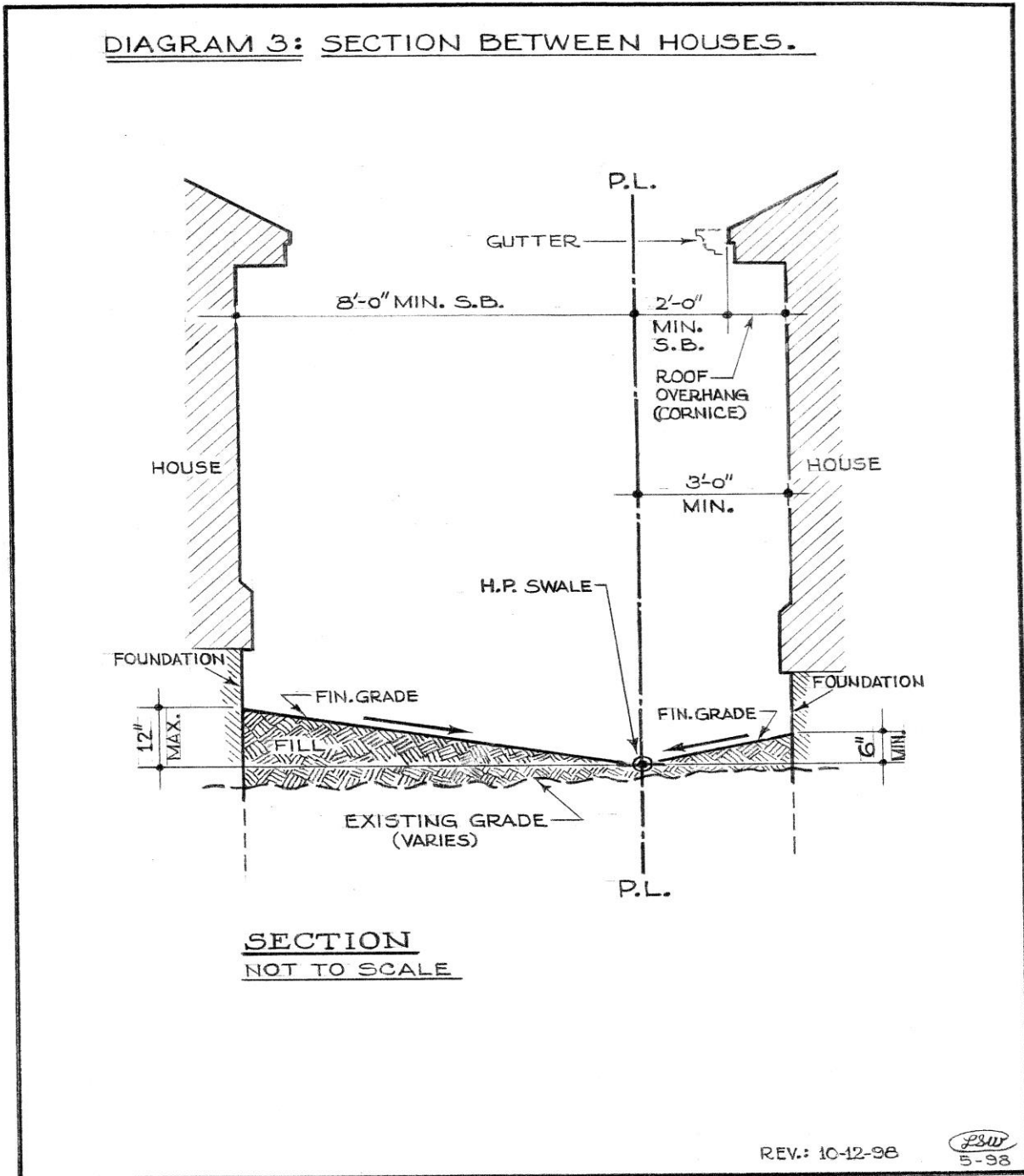
Diagram 3: Section Between Houses
